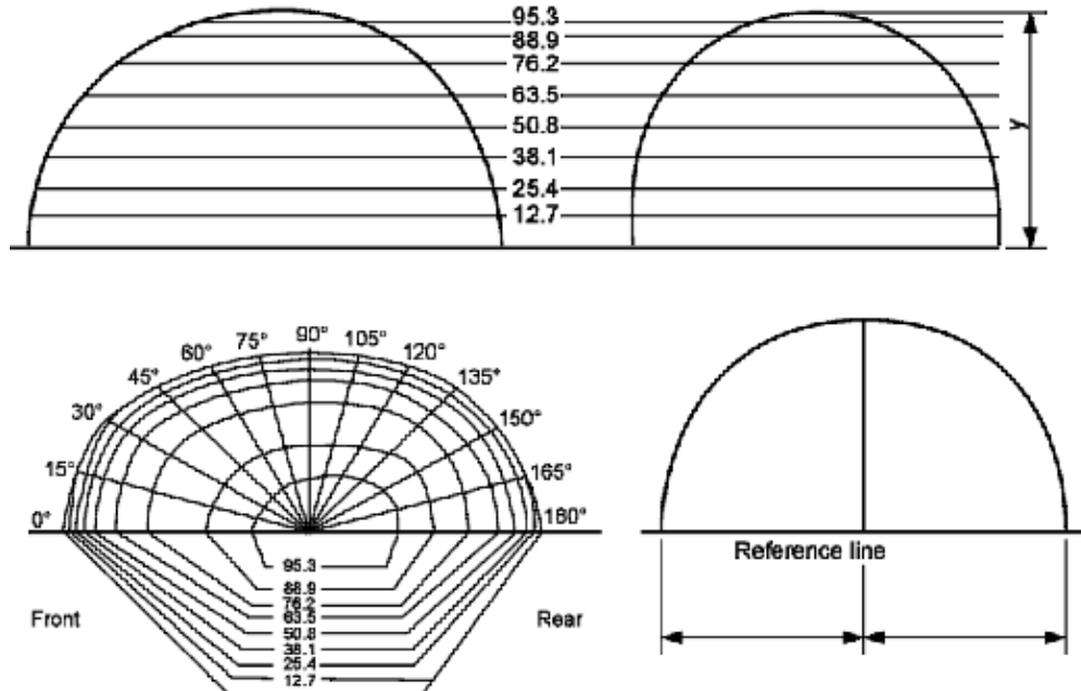
Dimensions of upper part of headforms (to be consulted in conjunction with annex 4, figure 3)
